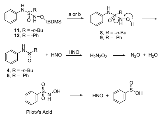
Scheme 3. Reagents: (a) TBAF; (b) CH 3 CO 2 H–H 2 O–THF.
