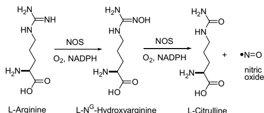
Scheme 1. NOS catalyzed oxidation of L-arginine to NO.
